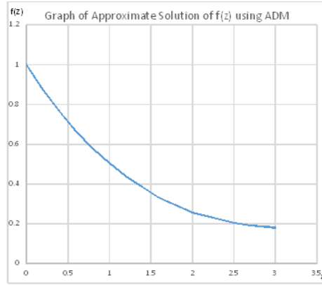
Figure 1.2 Graph of Approximate solution of f(z) by ADM
