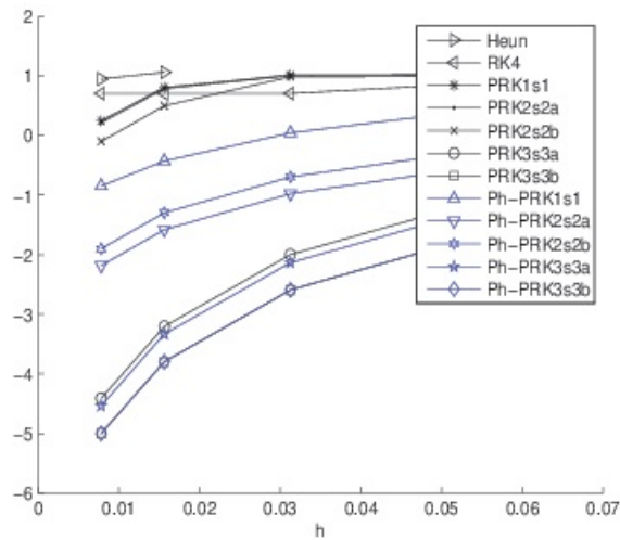
Figure 5: Problem 5.4. Accuracy comparison
