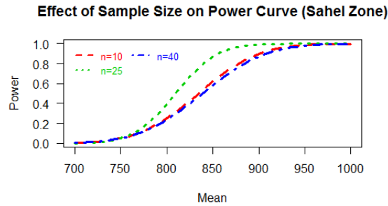
FIGURE 18. Sample Size Effect on Power Curve (Sahel Zone)
