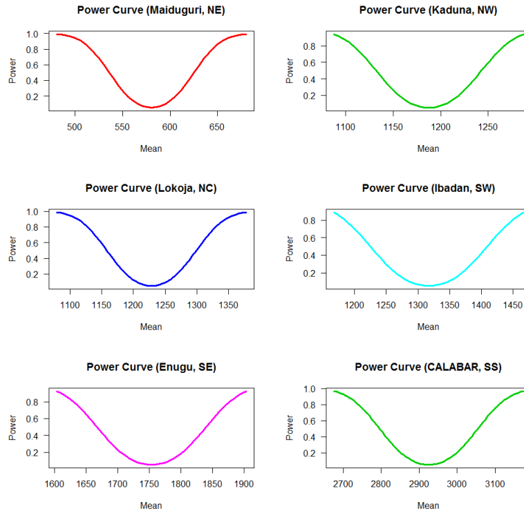
FIGURE 10. The Power Curve of the Two-tailed Test on Mean Annual Rainfall in the Geo-Political Zones
