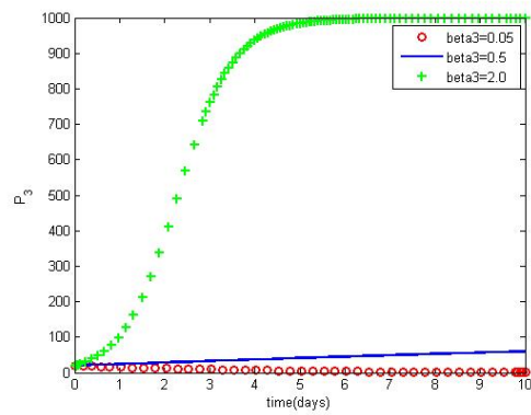
FIGURE 12. Variation of P_3 for different high values of \beta_3 .
