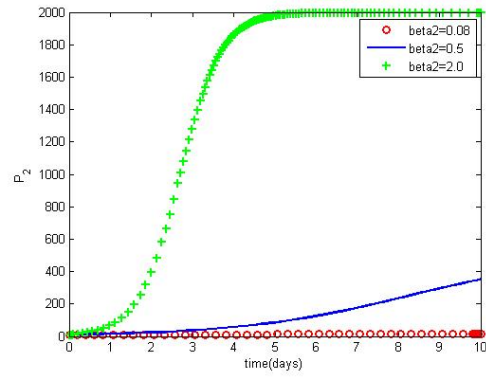
FIGURE 10. Variation of P_2 for different low values of \beta_2 .
