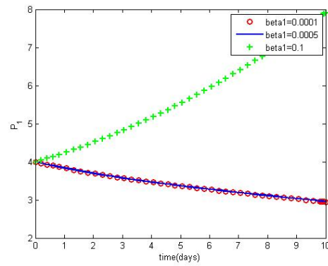
FIGURE 8. Variation of P_1 for different high values of \beta_1 .
