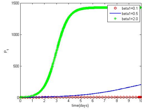
FIGURE 8. Variation of P_1 for different high values of \beta_1 .
