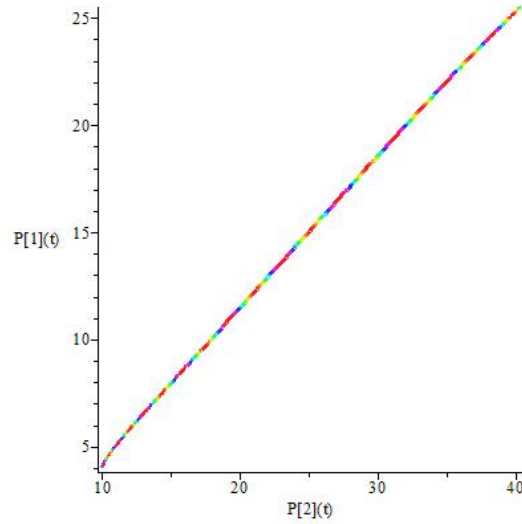
FIGURE 4. The phase portrait for the two( P_1 and P_2 ) species Lotka-Volterra model (6).
