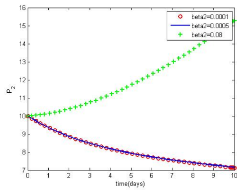
FIGURE 10. Variation of P_2 for different low values of \beta_2 .
