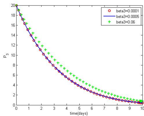
FIGURE 12. Variation of P_3 for different high values of \beta_3 .
