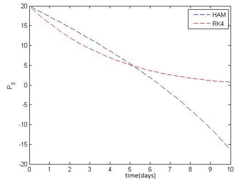
FIGURE 7. Plot of 9 th approximation for P_3 against time with HAM and ode45.
