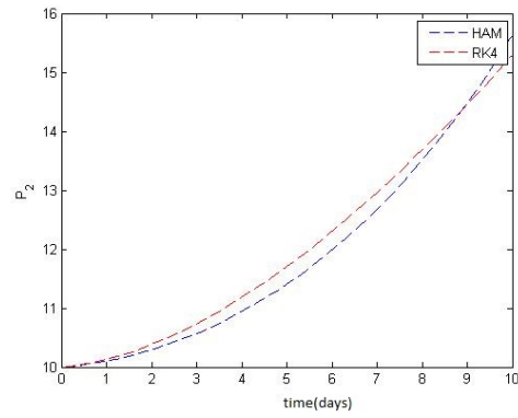
FIGURE 6. Plot of 9 th approximation for P_2 against time with HAM and ode45.
