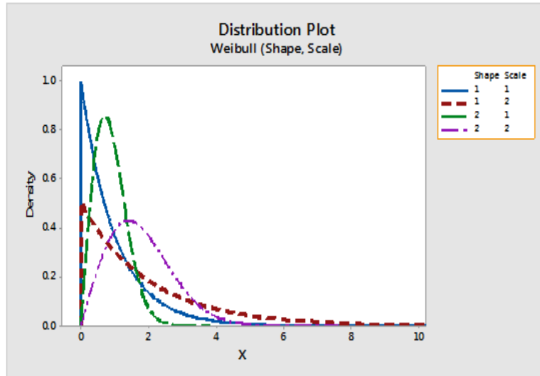
Figure 1: Distribution plot of Weibull distribution using different shape and scale parameters
