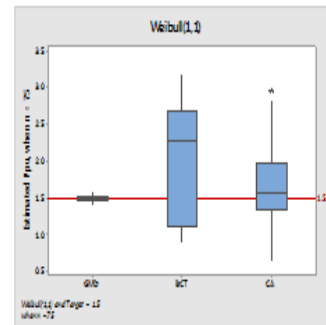
Figure 5: Weibull(1,1), target Ppu 1.5 and n=75
