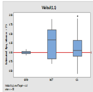
Figure 4: Weibull(1,1), target Ppu 1.0 and n=75
