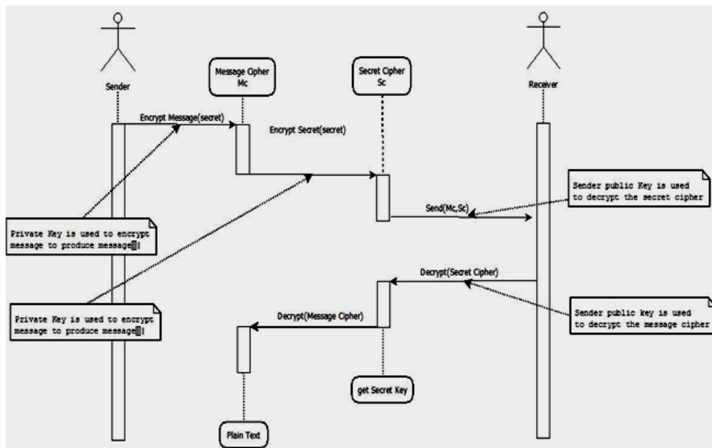
Sequence Diagram of the system
