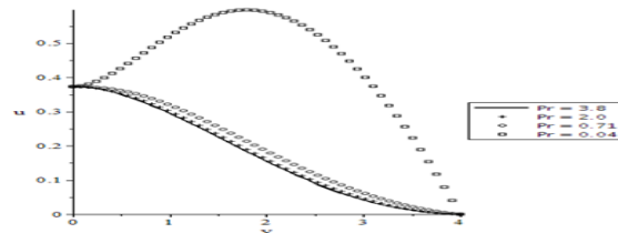
Figure 7: Velocity profile for Pr when \alpha = 3 , Mn = 0.5 , \lambda = 10 and N = 10
