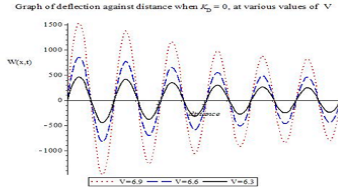
Figure 3.2: Effect of Speed of the Moving load on the Beam when K_D=0
