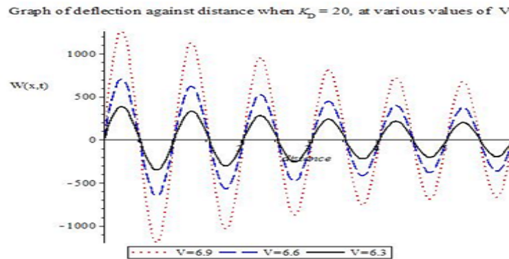
Figure 3.3: Effect of Speed of the Moving load on the Beam when K_D = 20
