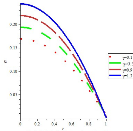
Fig.2: Velocity Profile for various values of \gamma
