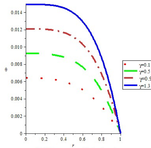
Fig.3: Temperature profile for values of \gamma
