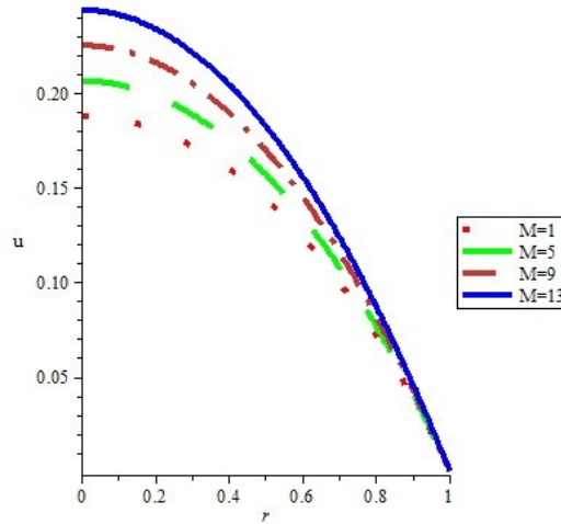
Fig 1: Graph of Velocity against Distance for various values of the Magnetic parameter
