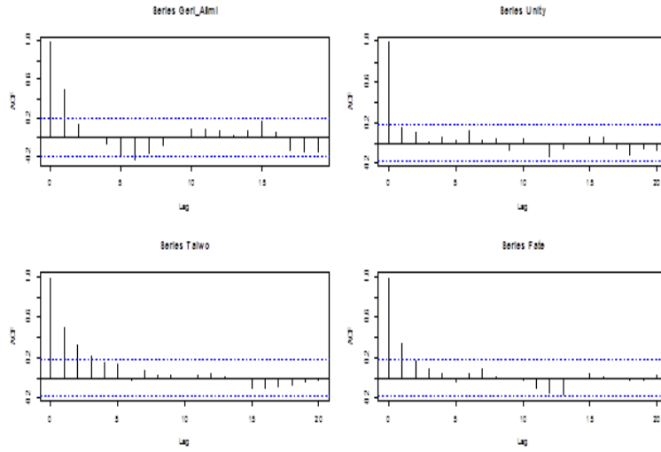
Figure 2: ACF plots of the Generating plants Noise from Different Locations
