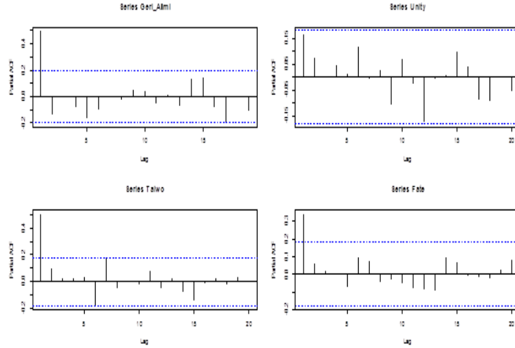
Figure 3: PACF plots of the Generating plants Noise from Different Locations
