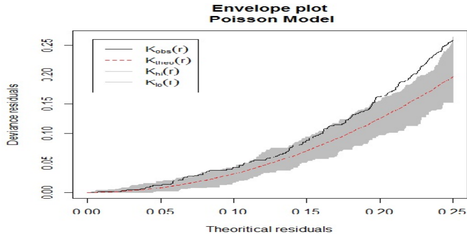
Figure 4: Envelope plots for the data set with clear signs of overdispersion with theoretical 95% confidence bands.
