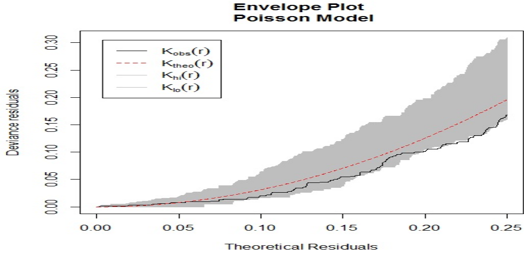
Figure 2: Envelope Plot of theoretical 95% confidence bands for Poisson Model
