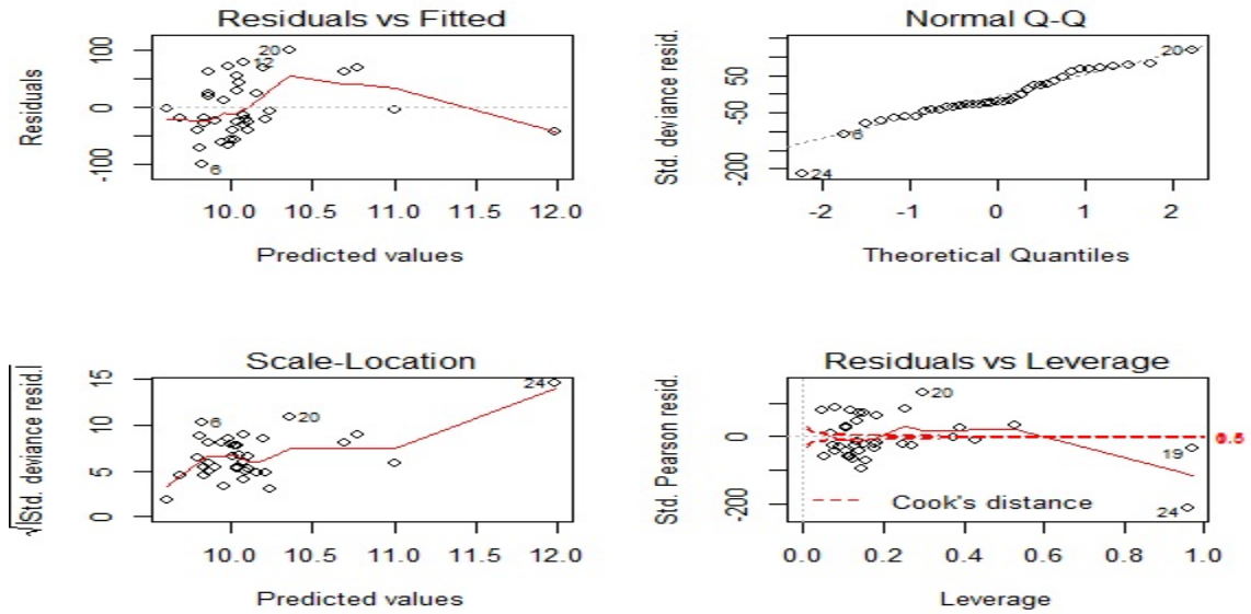
Figure 1: A Plot of Poisson Model for Estimating Infant Mortaliy in Nigeria.
