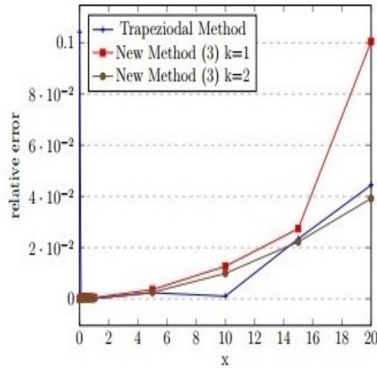
Figure 12: Comparison Graph of Relative Error for y_1(x) in Example 4
