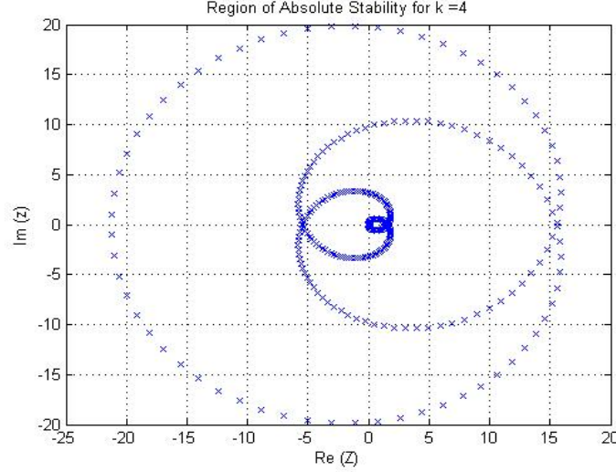
Figure 4: Stability Domain for k=4
