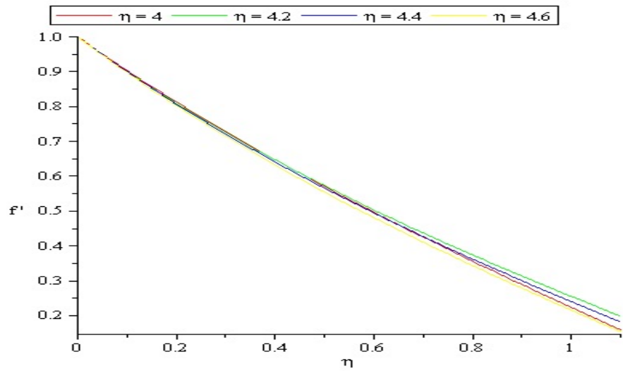
Graph of velocity profile f'(\eta) against (\eta) for \alpha = 4, 4.2, 4.4 and 4.6 keeping Gr = 0.1 and \eta = 0.2
